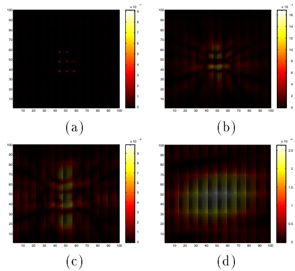
Fig. 8. The magnitude of the horizontally polarized electric field at a distance z from the slot array surface with one of the amplifier off: (b) z = \lambda/4 . (c) z = \lambda/2 . (d) z = 3\lambda .
