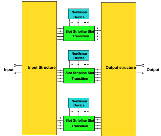
Fig. 3. Network model of large partitioned electromagnetic system.
