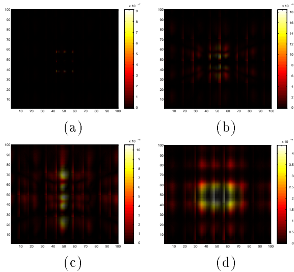
Fig. 7. The magnitude of the horizontally polarized electric field at a distance z from the slot array surface: (b) z = \lambda/4 . (c) z = \lambda/2 . (d) z = 3\lambda .
