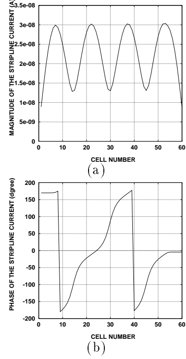
Fig. 5. The magnitude of the electrical current on the stripline at 10 GHz: (a) magnitude; and (b) phase.
