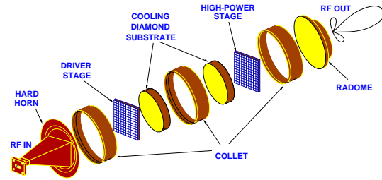
Fig. 1. Quasi-optical power combiner.
